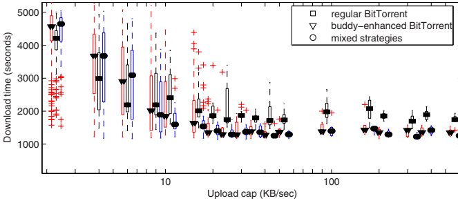
Fig. 6. Download completion time for leechers
