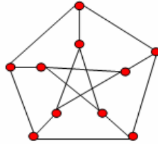
Fig. 2. Petersen graph
