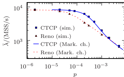
Fig. 4. Average Throughput
