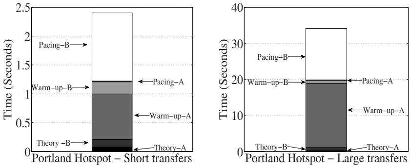
Fig. 6. Application impact for the Portland trace
